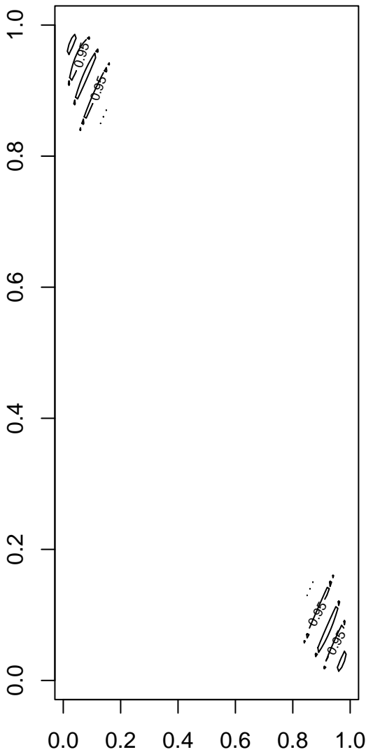
Coverage for score interval
