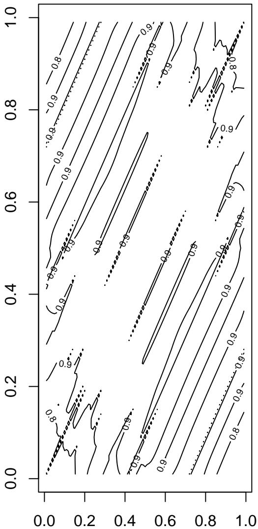
Coverage for wald interval
