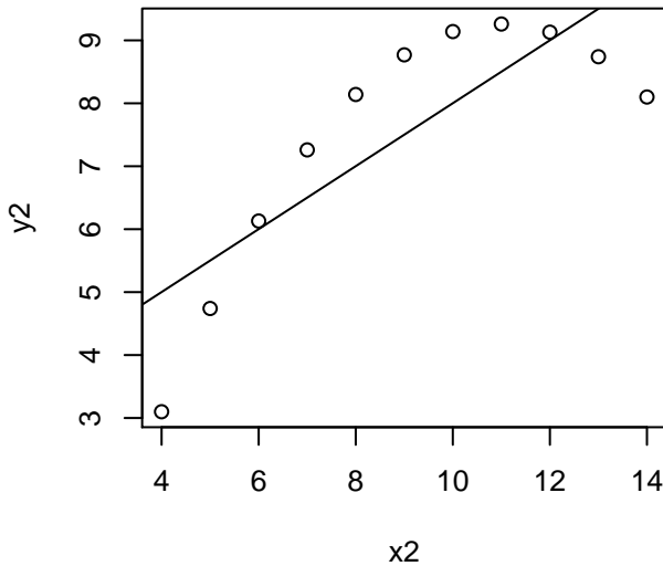
Linear Model Wrong
