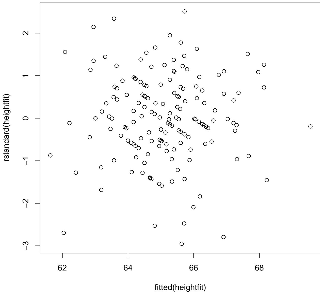
Residual plot for daughter height based on both parent heights
