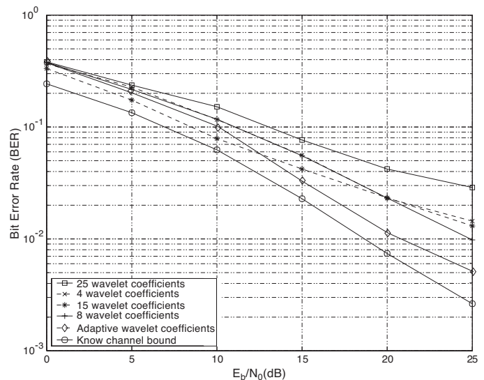
Fig. 3. BER performance of the SMC receiver using fixed number (e.g., 4, 8, 15, and 25) of wavelet coefficients and the adaptive wavelet-based SMC receiver. The channel is flat-fading with f_dT = 0.005 . The delayed-weight method is used with \delta = 6 .
