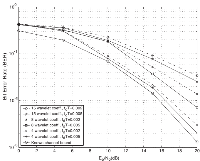
Fig. 8. BER performance of the SMC receiver using fixed number (e.g., 4, 8, and 15) of wavelet coefficients under different Dopplers. The channel is frequency-selective fading with L = 2 . The delayed-sample method is used with \Delta = 2 .
