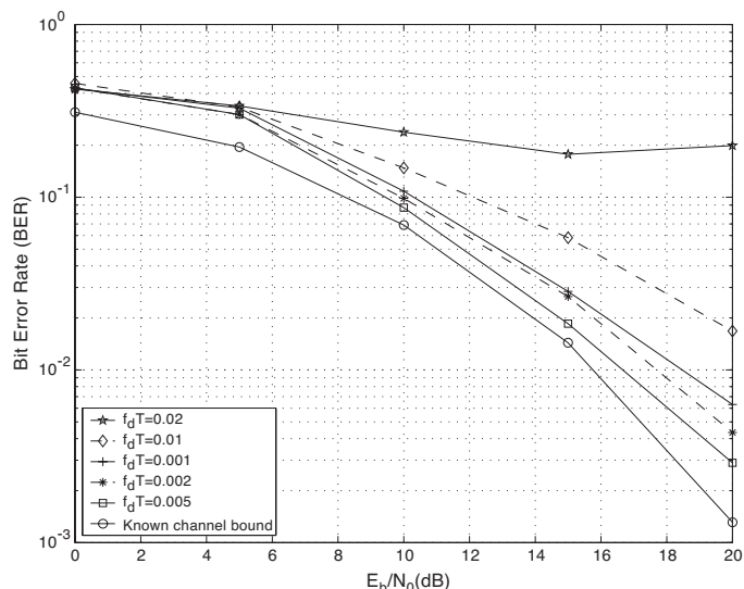
Fig. 9. BER performance of the adaptive shrinkage SMC receiver. The channel is frequency-selective fading with L = 2 . The delayed-sample/delayed-weight methods are used with \Delta = 2 and \delta = 6 .
