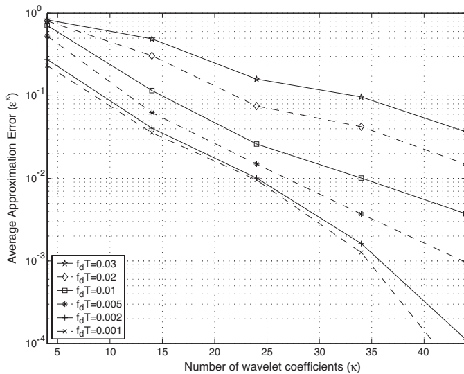
Fig. 1. Average approximation error versus the number of wavelet coefficients in the wavelet representation of the fading processes. The Daubechies filter with order 2 is used.
