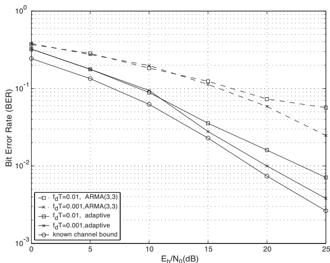
Fig. 7. BER performance of the adaptive shrinkage SMC receiver and the mixture Kalman filter with statistically approximated ARMA models. The channel is flat fading under different Dopplers. The delayed-weight method is used with \delta = 6 .
