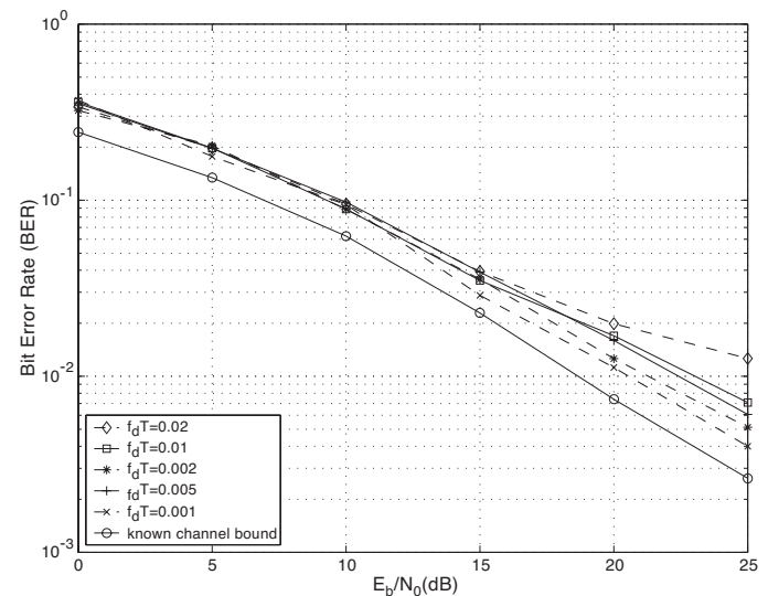
Fig. 6. BER performance of the adaptive shrinkage SMC receiver. The channel is flat fading under different Dopplers. The delayed-weight method is used with \delta = 6 .
