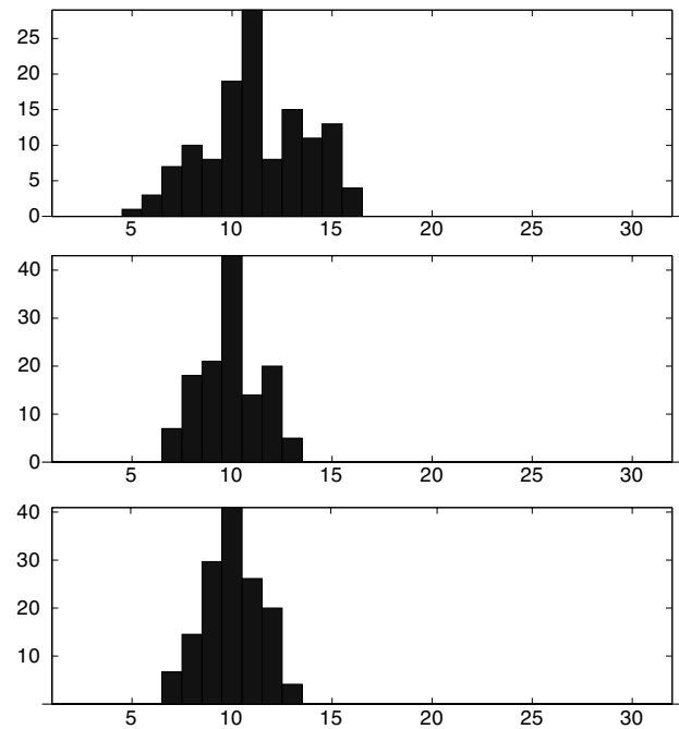
Fig. 5. Histogram for the number of the wavelet coefficients associated with the sample streams at times t = 20 (top), t = 40 (middle), and t = 64 (bottom) for f_d T = 0.005 and E_b/N_0 = 10 dB. The result is the average over 100 simulations.
