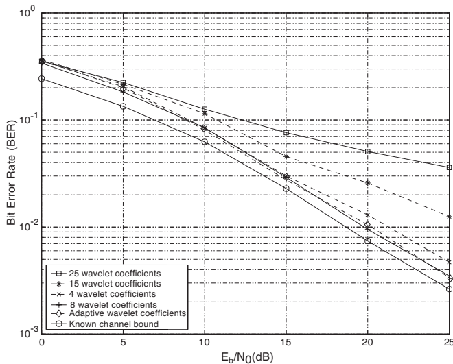
Fig. 4. BER performance of the SMC receiver using fixed number (e.g., 4, 8, 15, and 25) of wavelet coefficients and the adaptive wavelet-based SMC receiver. The channel is flat-fading with f_d T = 0.01 . The delayed-weight method is used with \delta = 6 .
