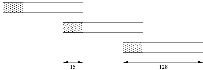
Fig. 2. Frame structure for the wavelet-based SMC receivers. The block size is 128, and the adjacent blocks overlap by 15 symbols.
